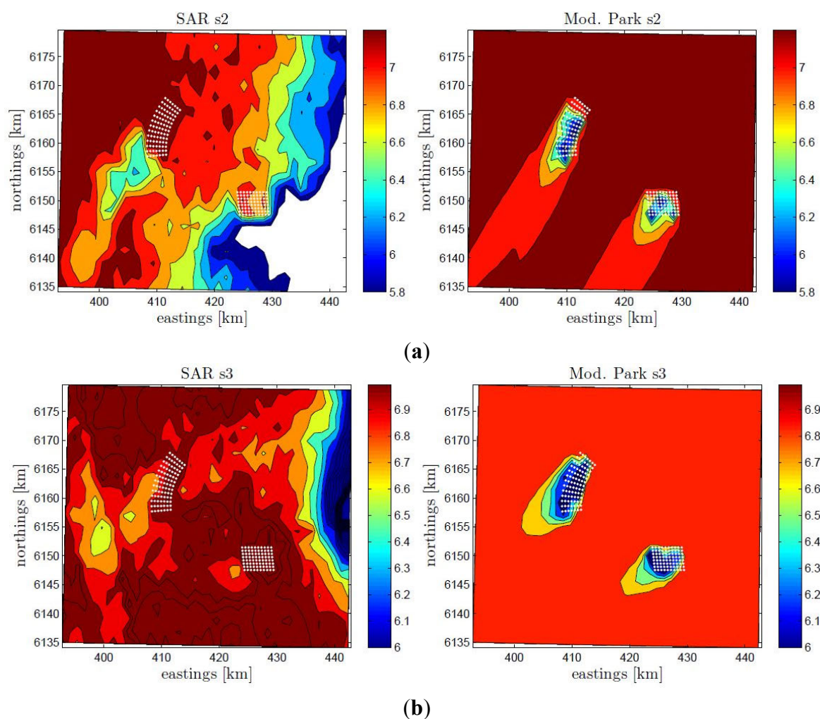
Figure 5. Average wind speed based on satellite SAR ( left ) and modified PARG wake model results ( right ) at 10 m height for the Horns Rev wind farm area for winds from Sector 2 ( a ) and Sector 3 ( b ). The color bar indicates wind speed in \text{m}\cdot\text{s}^{-1} .
